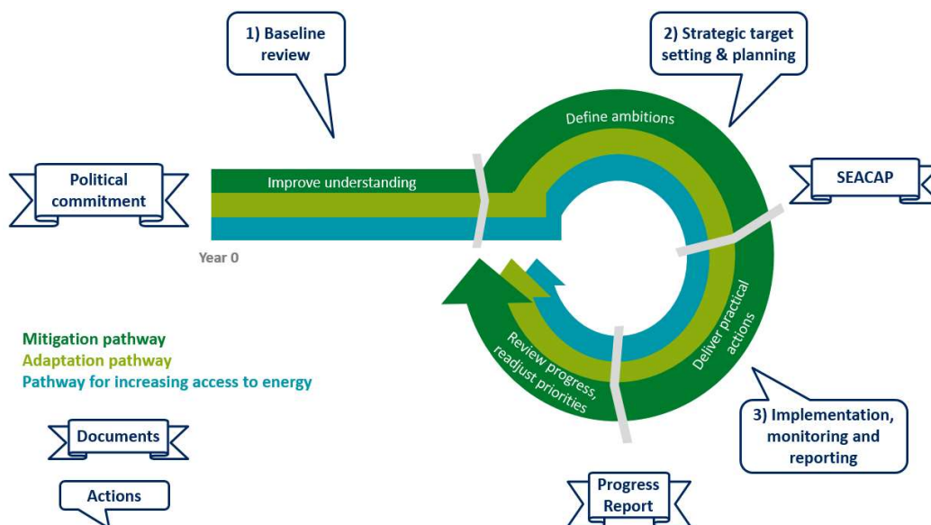
Figure 1: SEACAP Process
